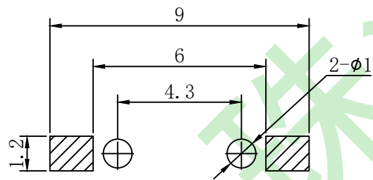
PCB焊接图 PCB. WELDING DRAWING
